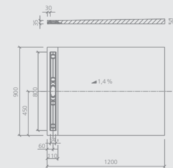
Fundo Riolito neo , rectangular
