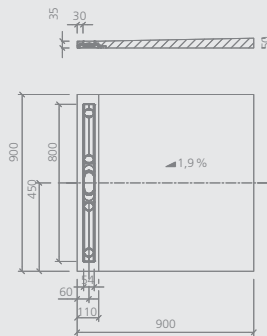
Fundo Riolito neo , square
