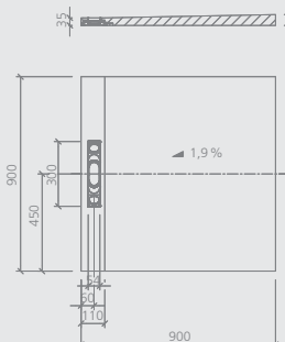
Fundo Riolito neo , square, with short channel
