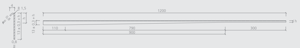
wedi Fundo Riolito neo slope profile wall, left-hand version
